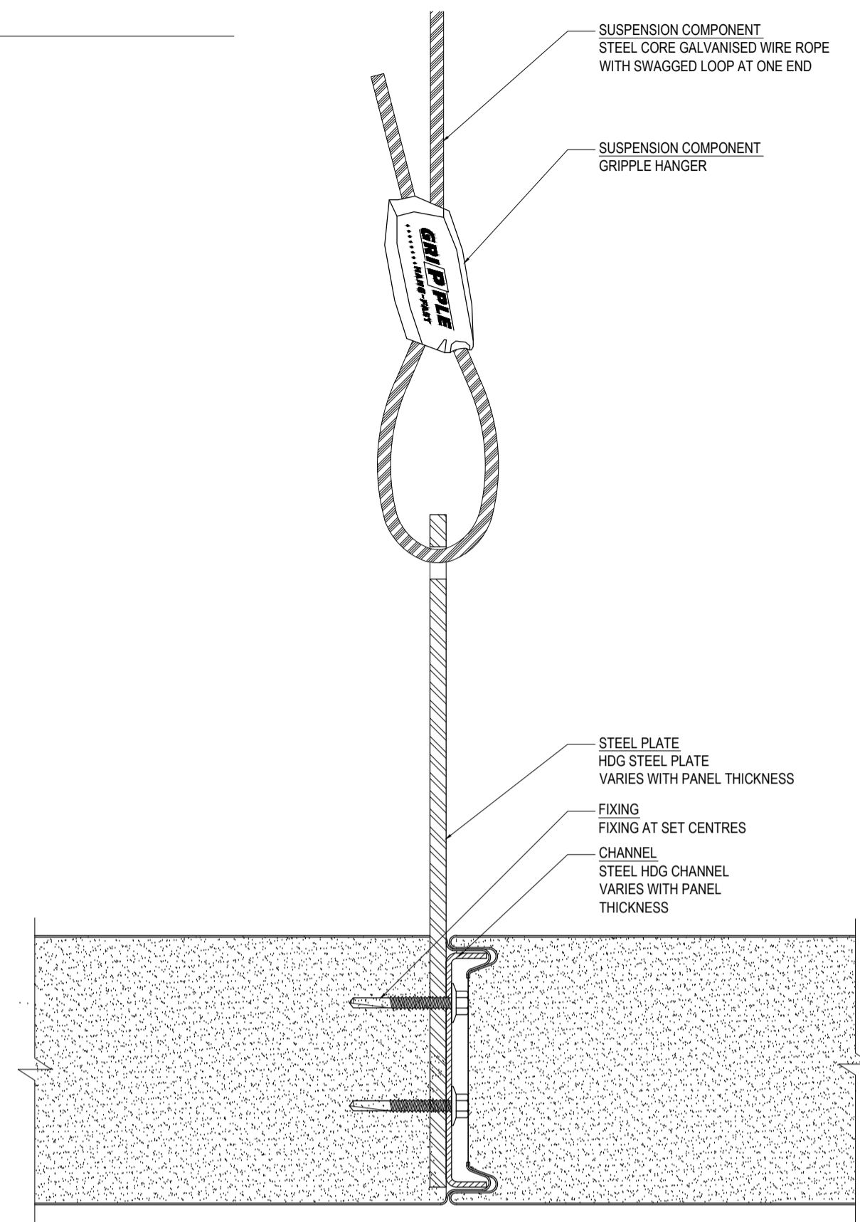
IWC-XCS-AT-20 SCALE 1:2
