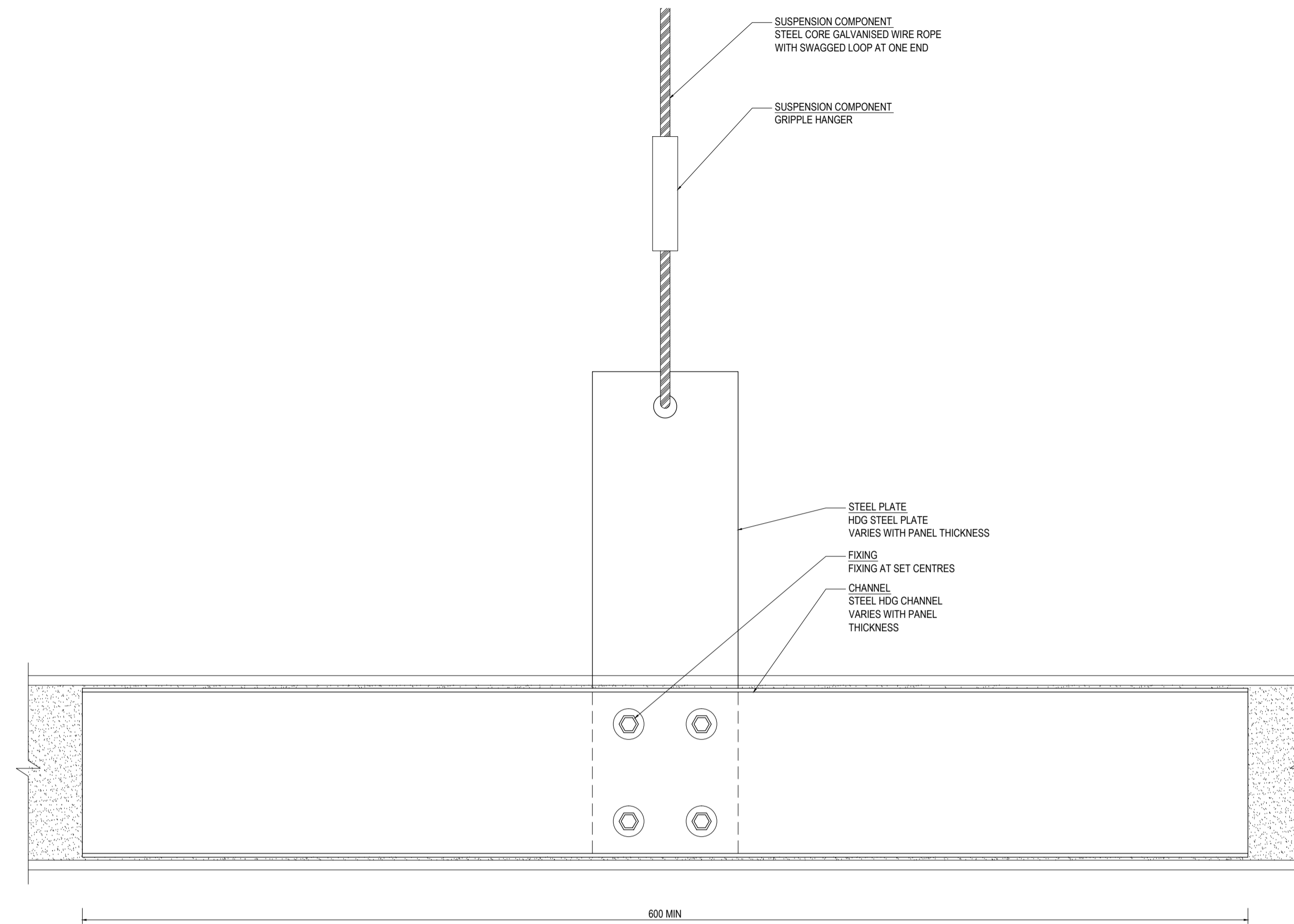
IWC-XCS-AT-21 SCALE 1:2
